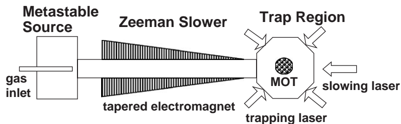
Fig. 1. Schematic of the proposed experimental apparatus for measuring krypton impurities.
