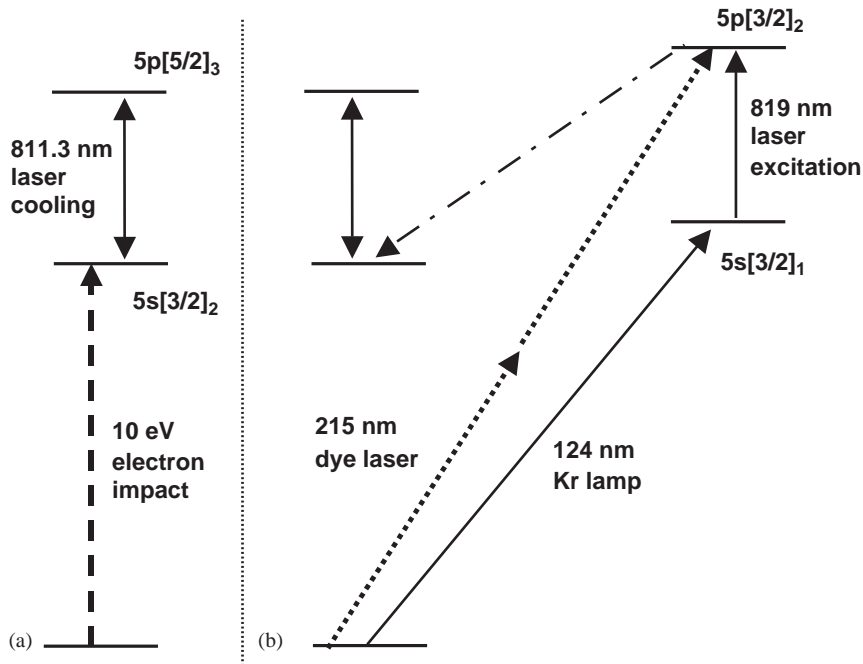
Fig. 2. The atomic levels of Kr. (a) Shows the energy levels relevant to atomic trapping of Kr^* , and (b) shows the energy levels relevant to resonant and non-resonant optical excitation of Kr^* .
